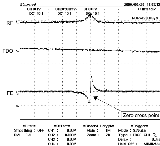
S-Curve of DVD Single Layered disc
